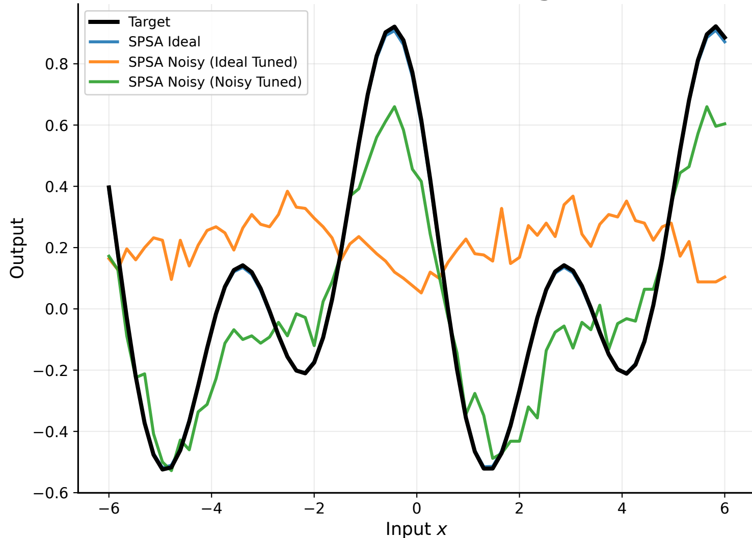
Model Predictions vs Target
